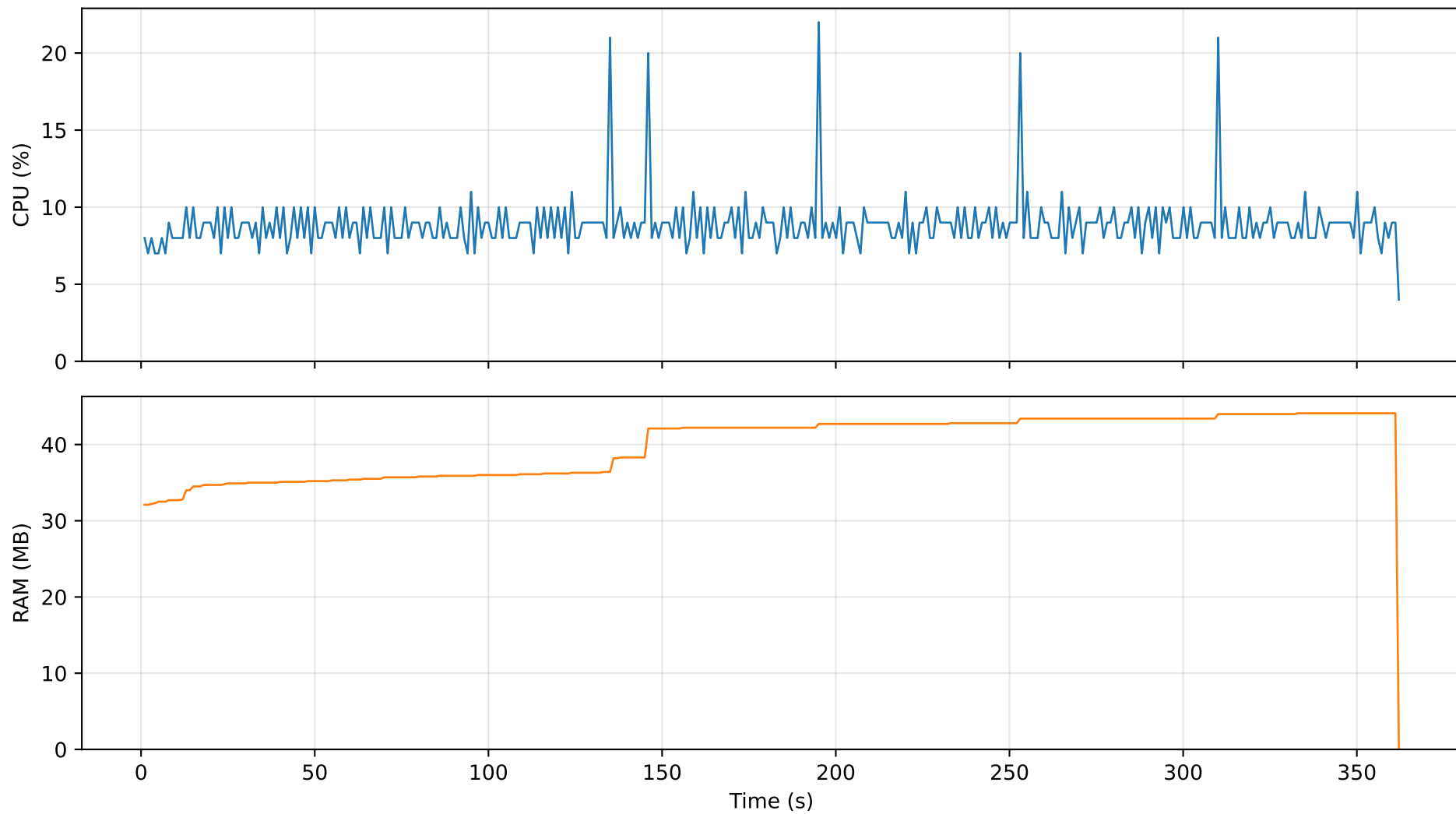
Resource Usage — 5pct_003
