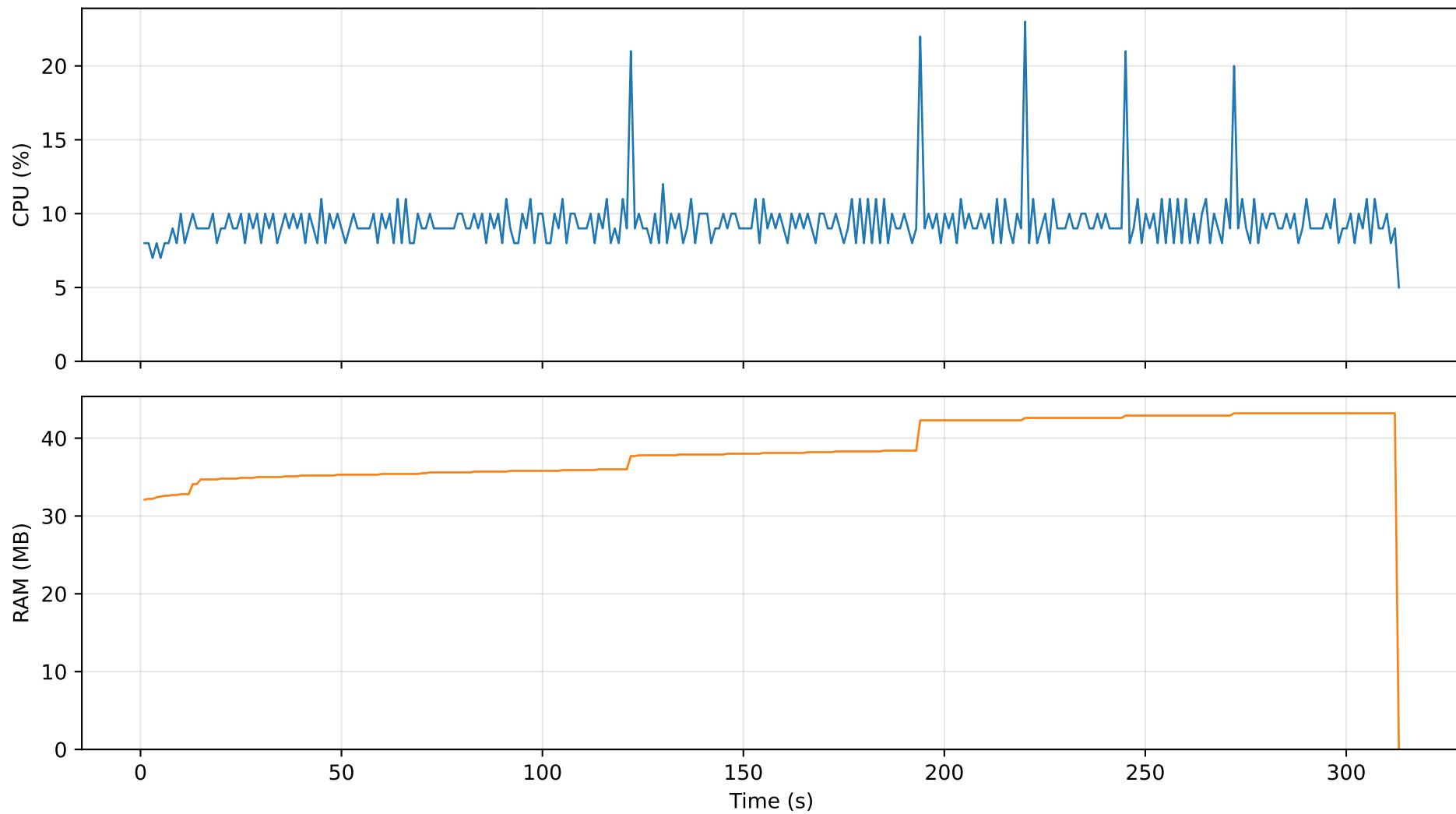
Resource Usage — 20pct_003
