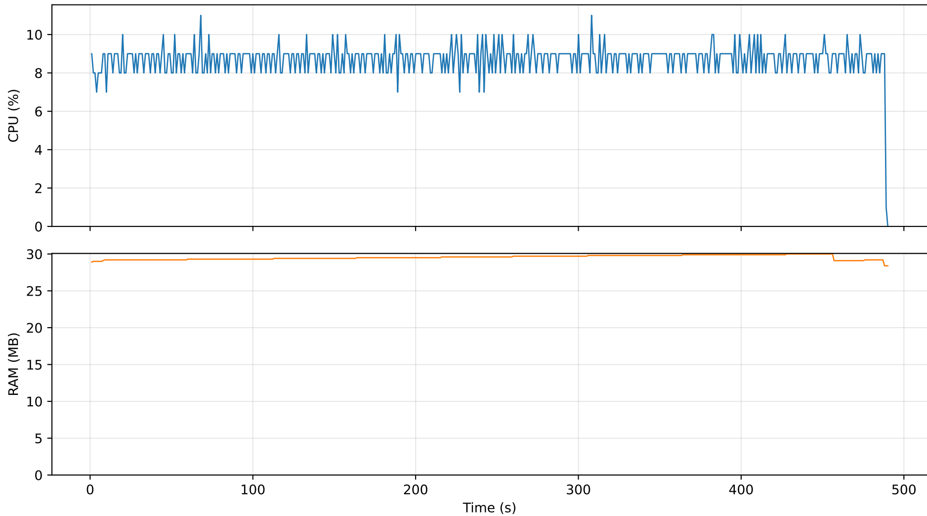
Resource Usage — 10pct_008
