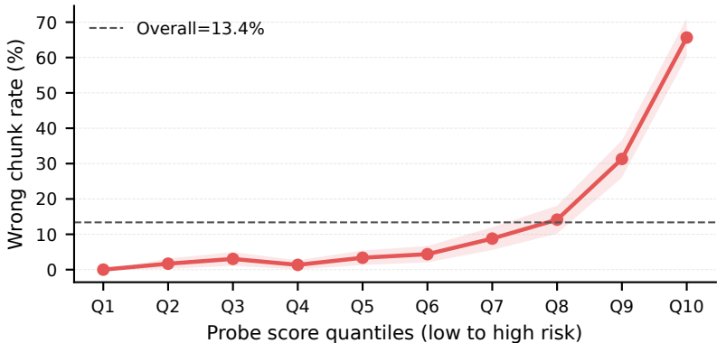
Error rate rises with hidden-state probe risk
