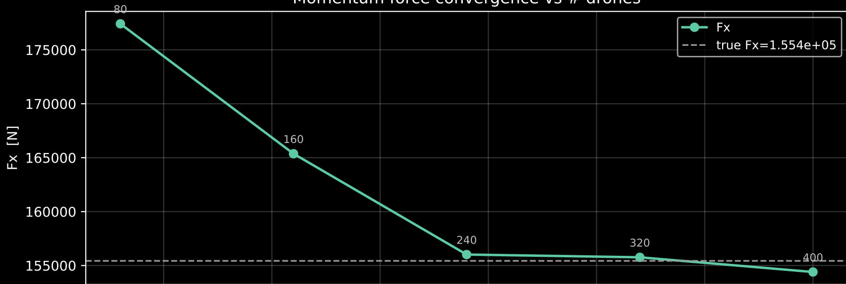
Momentum force convergence vs # drones
