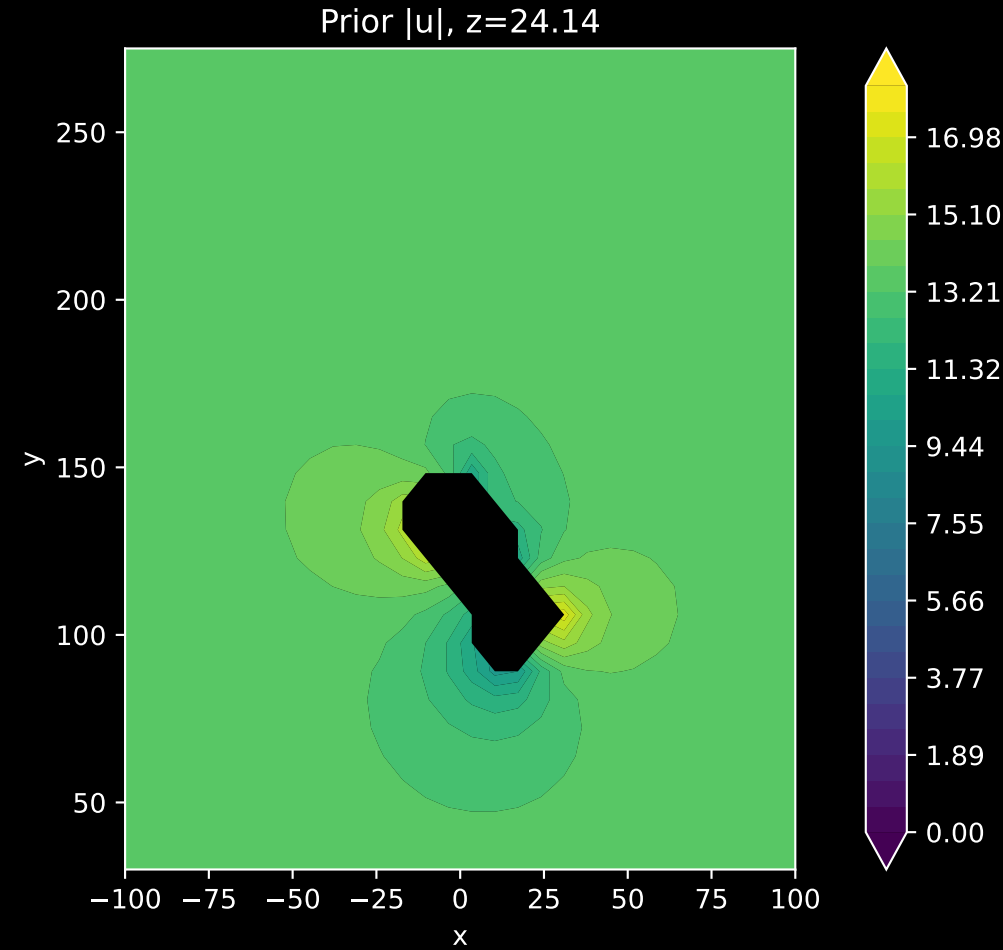
Prior - CFD |u| , z=24.14
