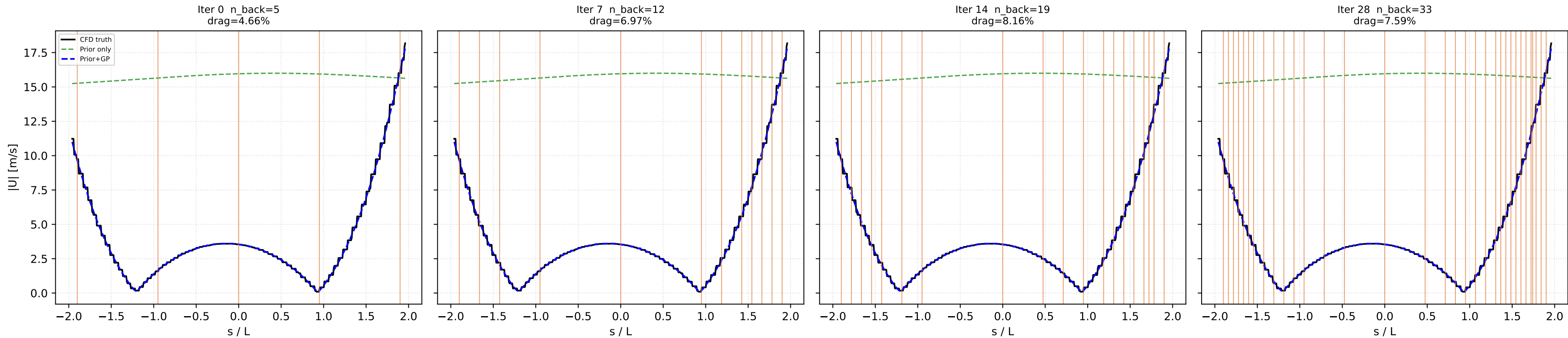
Back-face |U| : truth / prior / prior+GP Orange ticks = drones
