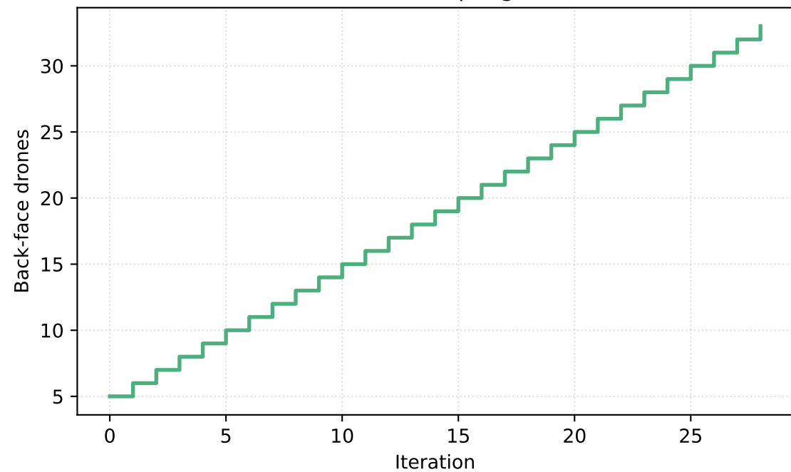
Back-face sample growth
