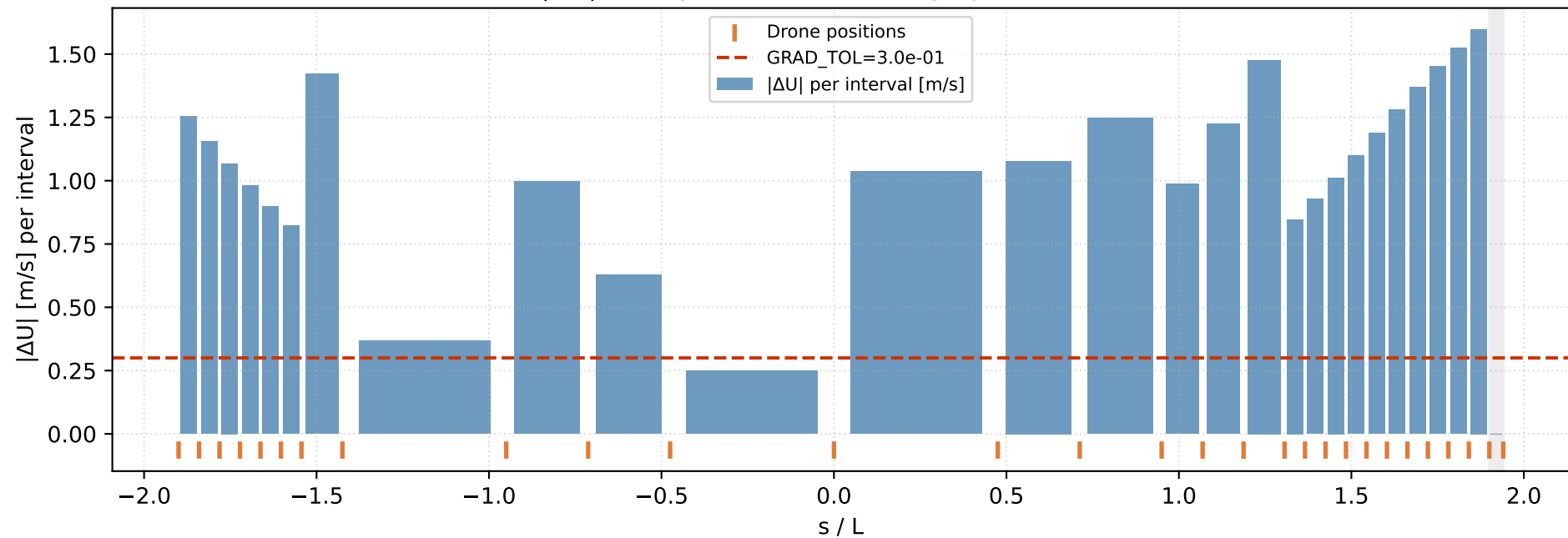
Back-face velocity jump per interval — final Bars = |\Delta U| ; orange ticks = drones; grey = min-width mask
