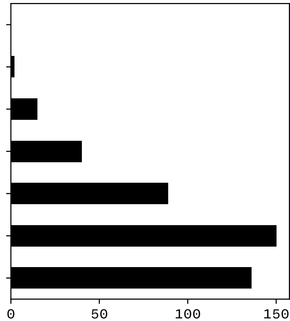
Devanagari
