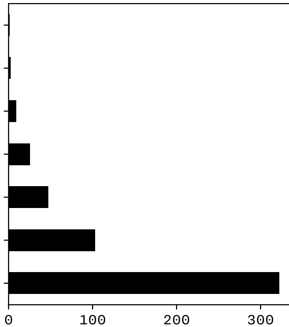
Cyrillic
