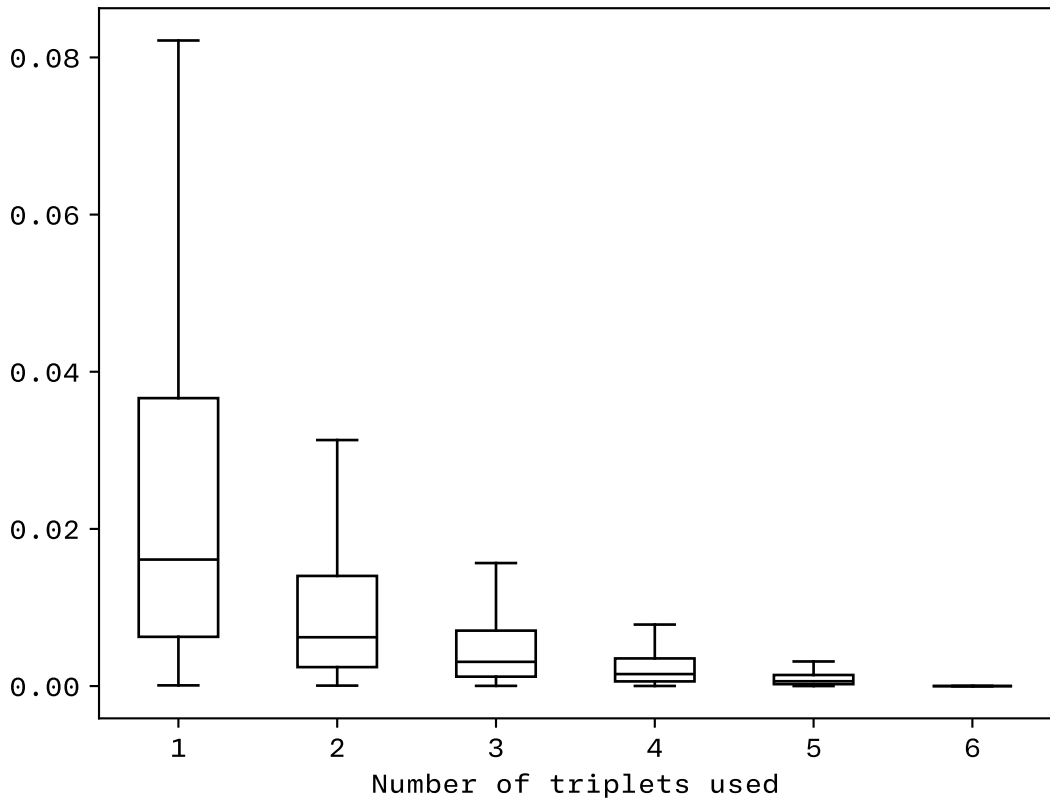
Pair-similarity variance
