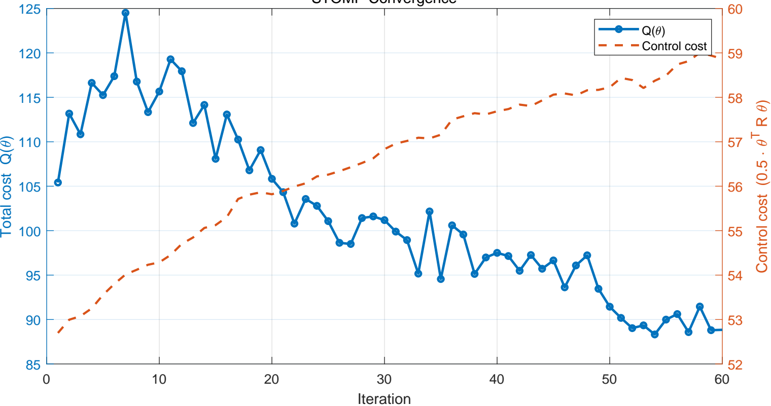
STOMP Convergence
