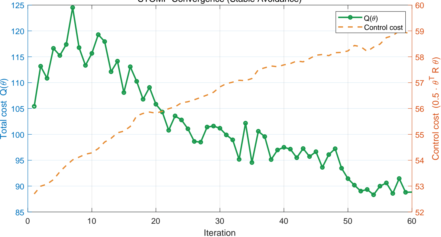
STOMP Convergence (Stable Avoidance)
