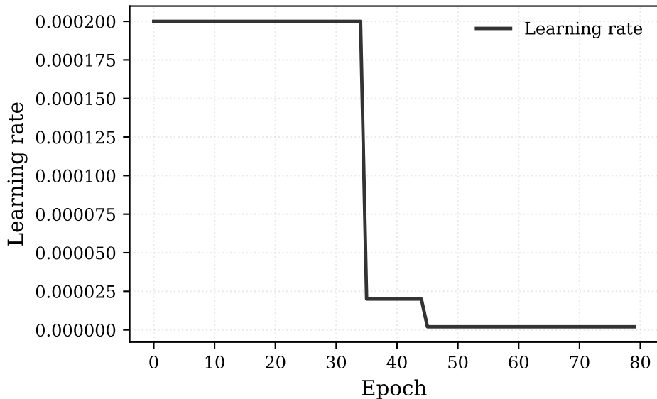
KITTI — Adam step LR schedule
