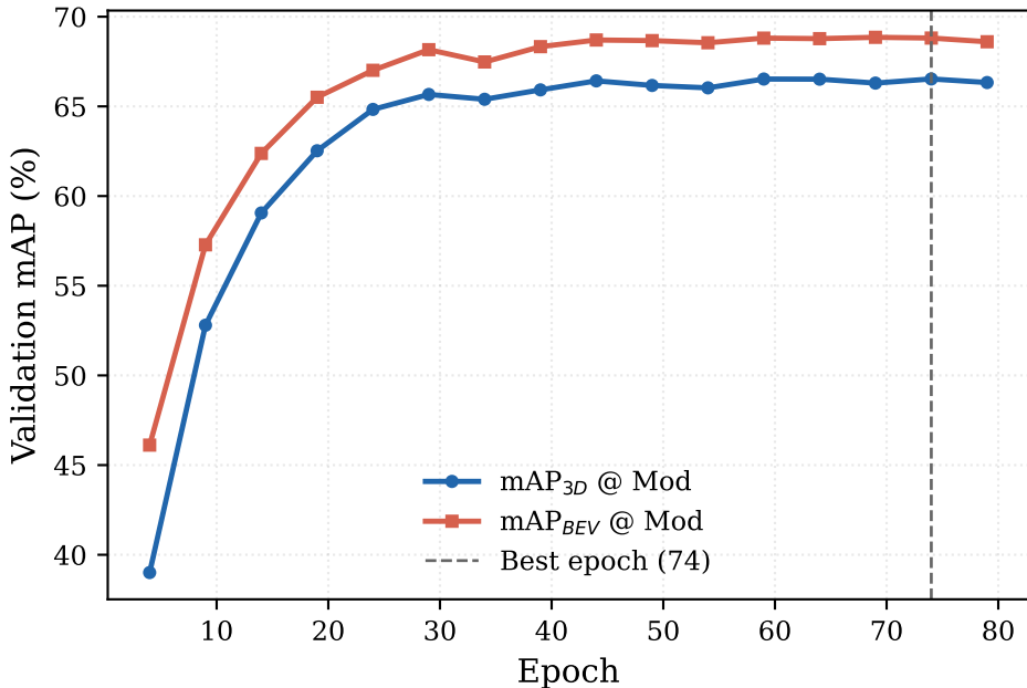
KITTI — validation mAP
