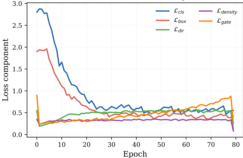
nuScenes — AG-DPE loss components
