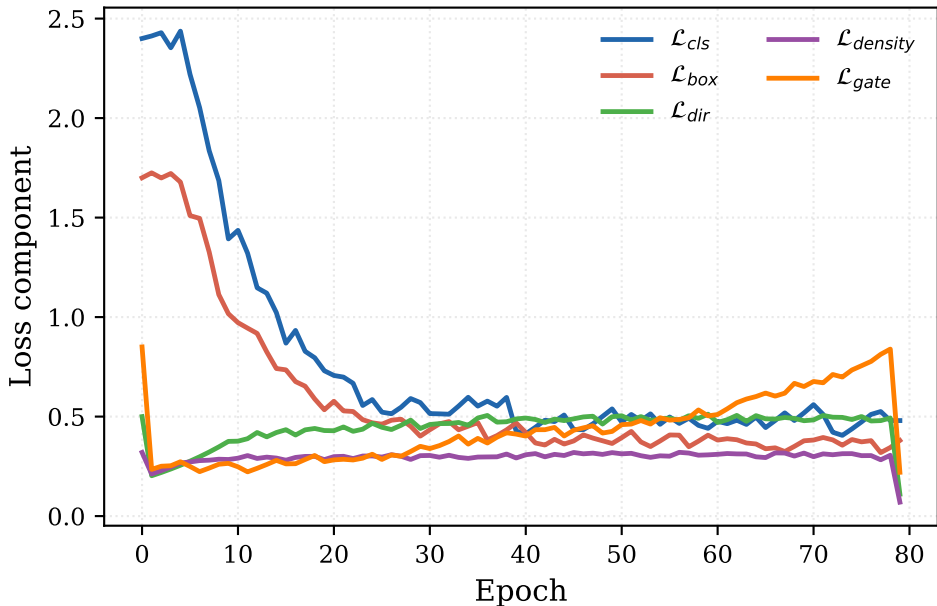
Waymo — AG-DPE loss components
