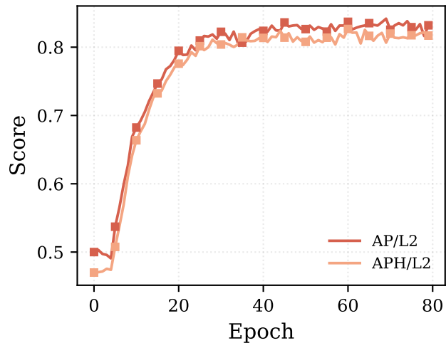
(c) Validation AP/APH (L2)
