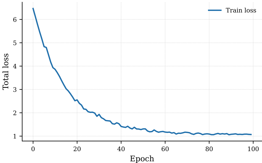
KITTI — DPCA-Net training loss
