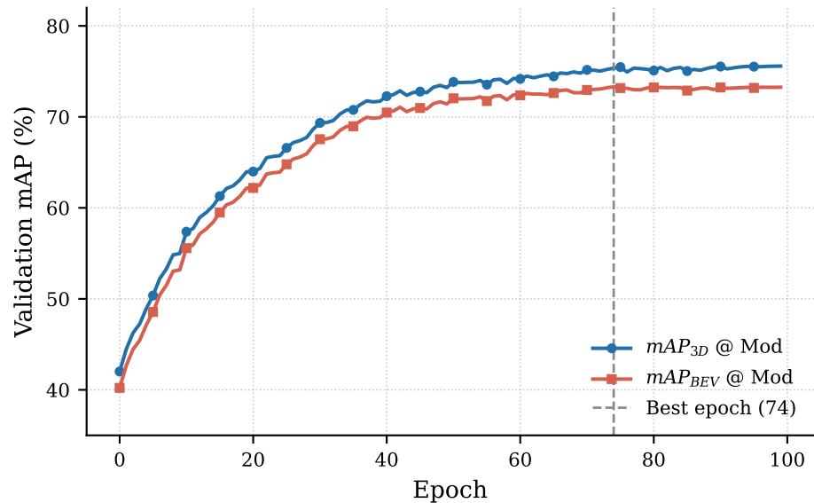
KITTI — validation mAP
