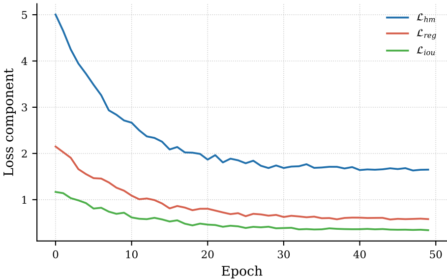
nuScenes — DPCA-Net loss components
