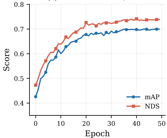
(c) Validation mAP / NDS
