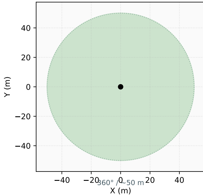
nuScenes
