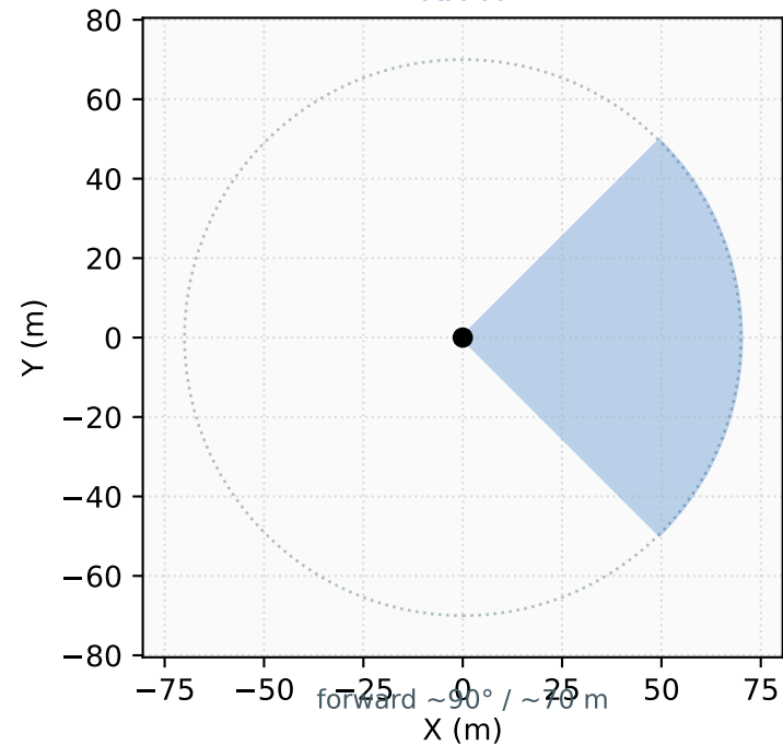
KITTI
