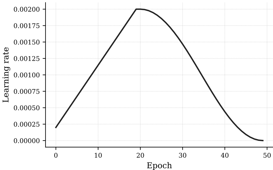
Waymo — AdamW one-cycle LR schedule
