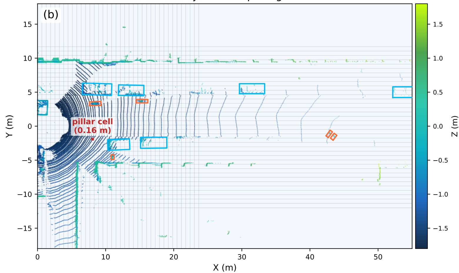
Bird's-Eye View + pillar grid
