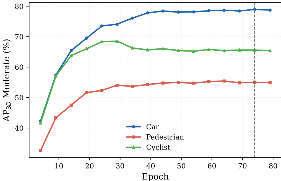
KITTI — per-class AP 3D
