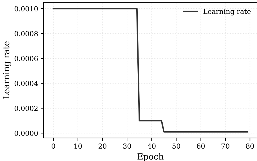
nuScenes — Adam step LR schedule
