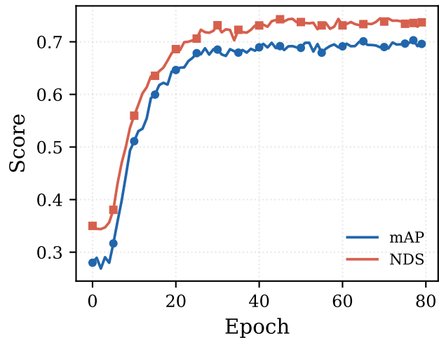
(c) Validation mAP / NDS
