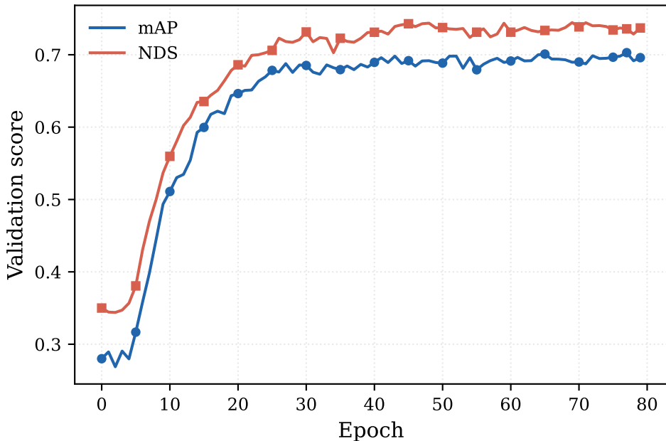
nuScenes — validation mAP / NDS
