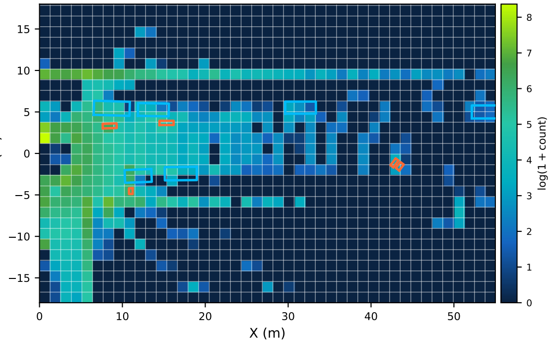
Coarse context grid (1.28 m)
