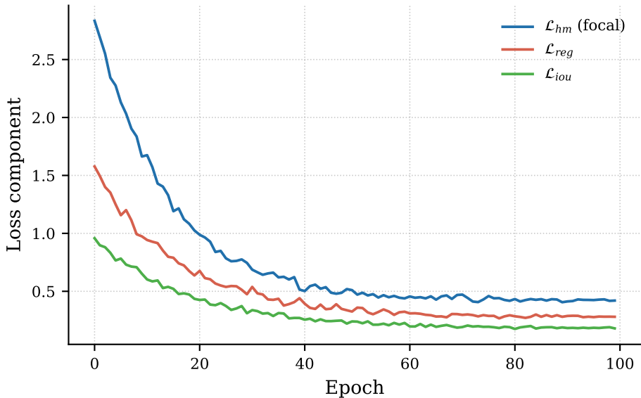
KITTI — DPCA-Net loss components
