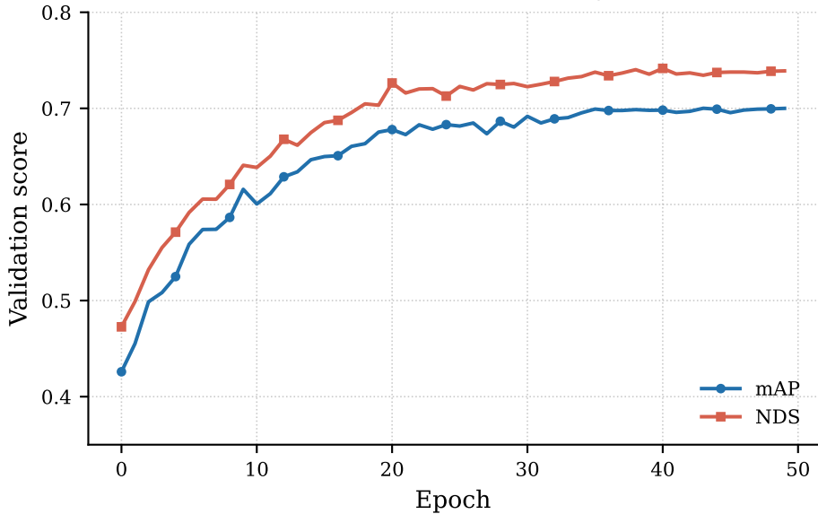
nuScenes — validation mAP / NDS
