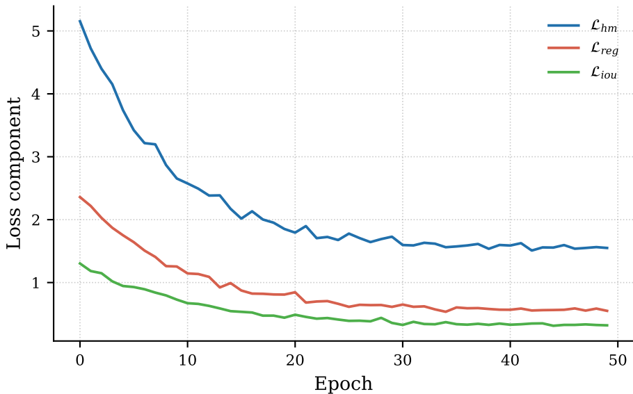
Waymo — DPCA-Net loss components
