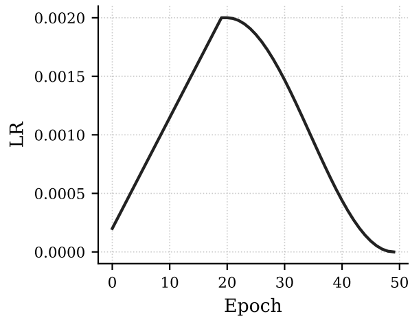
(b) Learning rate
