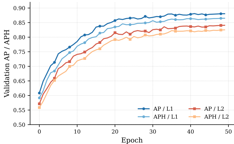
Waymo — validation AP/APH
