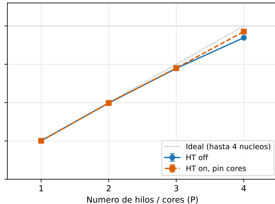
CMP: speedup
