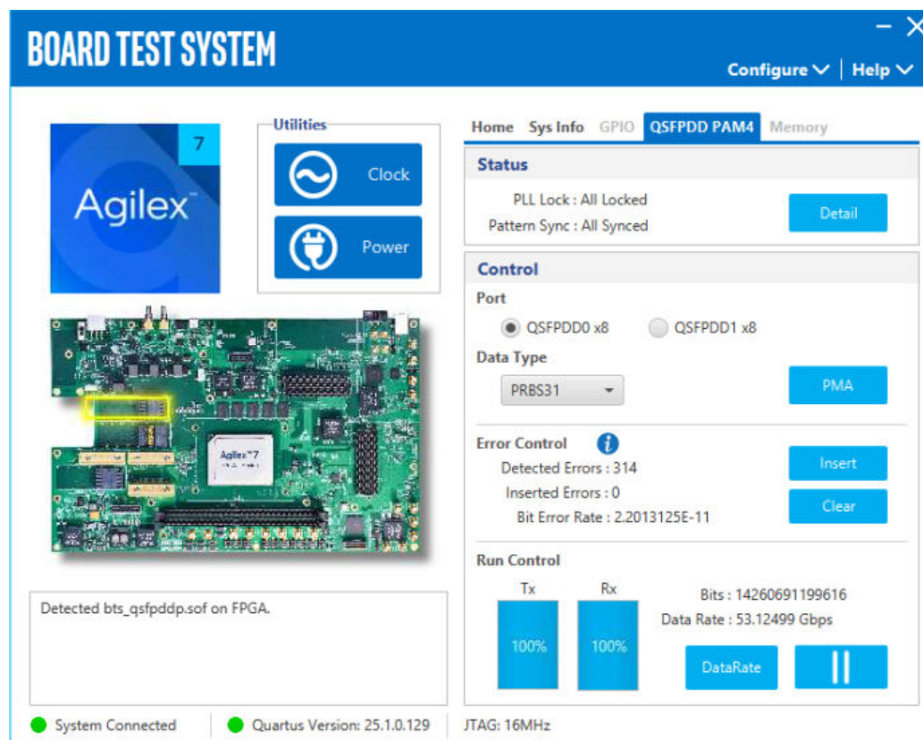
Figure 17. The QSFDD PAM4 Tab
