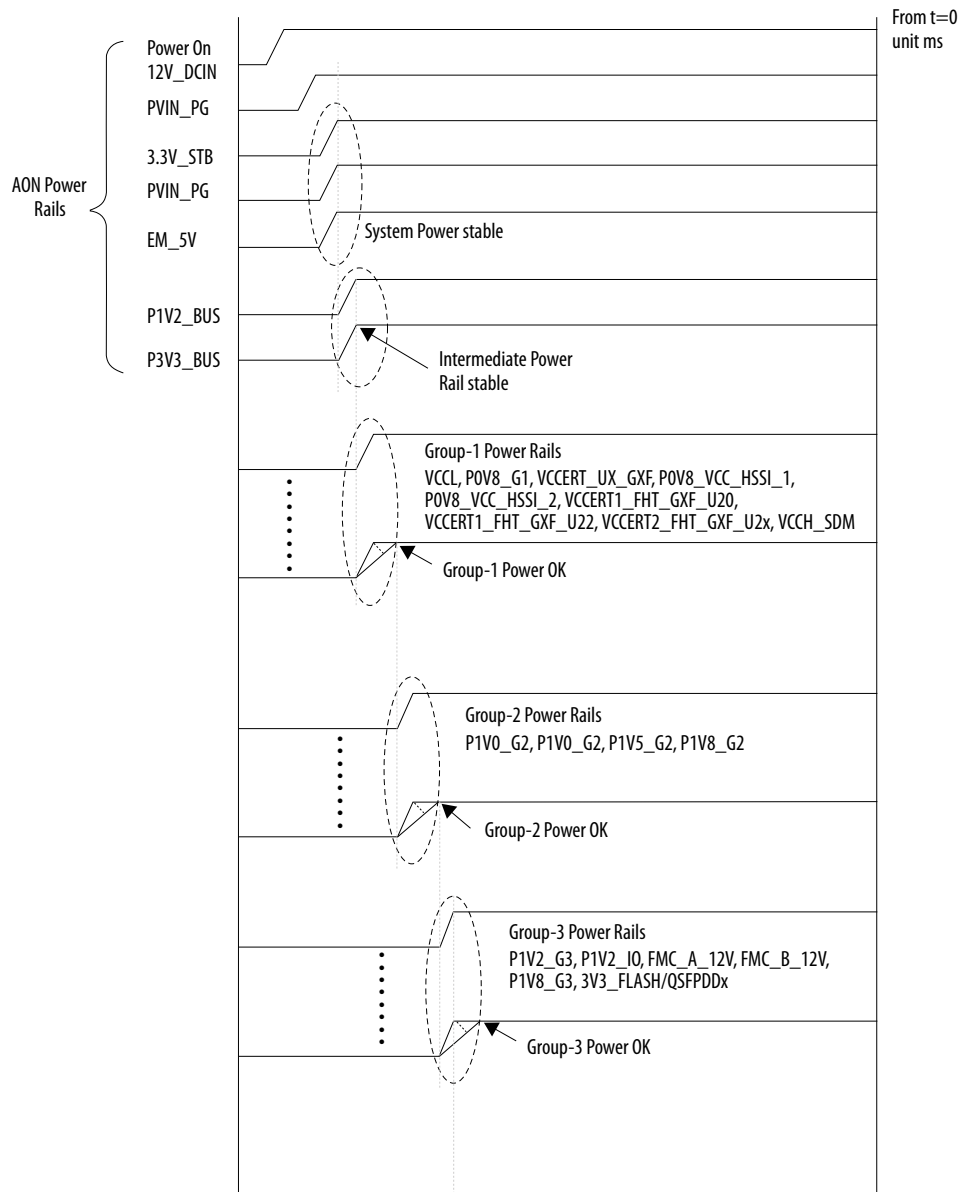
Figure 34. Power Sequence
