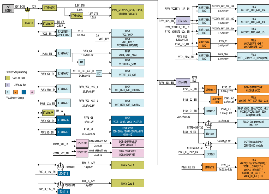
Figure 32. Power Tree (Power Solution 2 Board—non-Enpirion)
