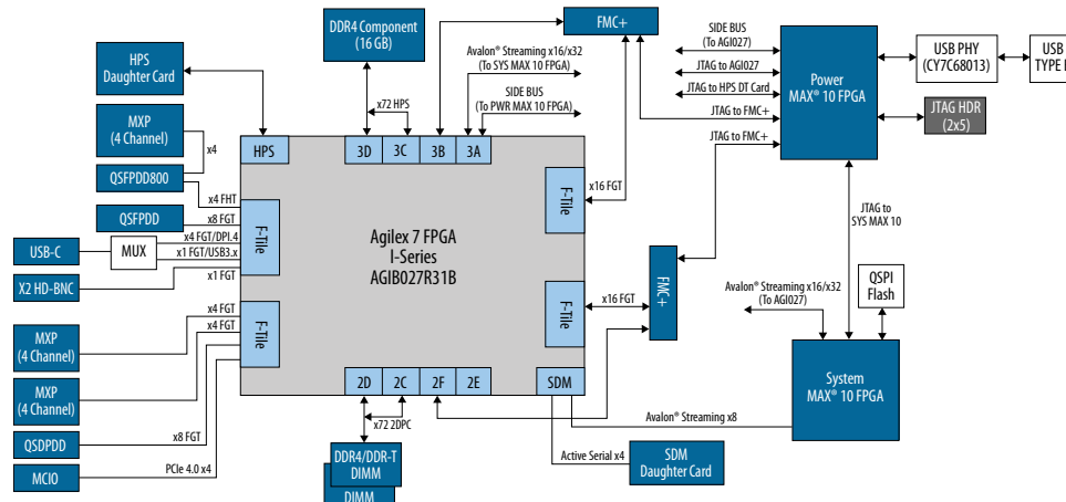
Figure 3. Agilex 7 FPGA I-Series Transceiver-SoC Development Kit Block Diagram
