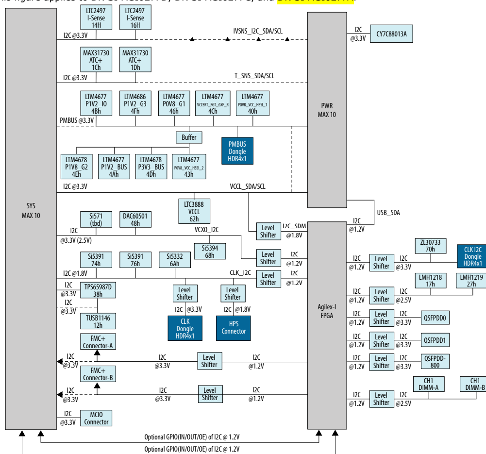
Figure 37. I 2 C Serial Bus (Power Solution 2 Board—non-Enpirion)
