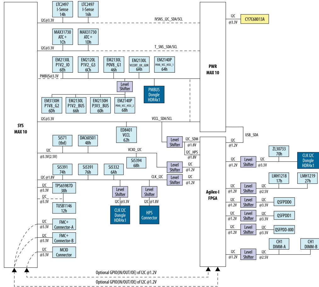
Figure 38. I 2 C Serial Bus (Power Solution 1 Board—Enpirion)
