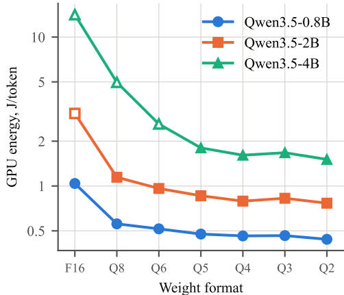
Decode (generation)
