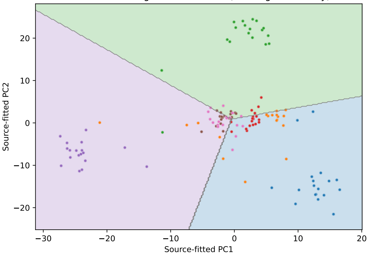
Original classifier on PCA plane; target points Slice/full-head agreement: 45.7% (not target accuracy)
