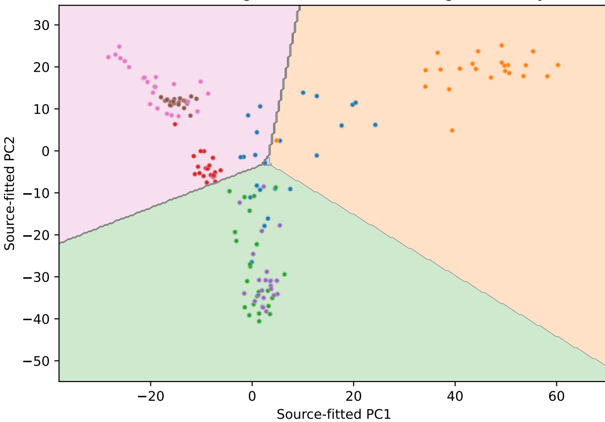
Original classifier on PCA plane; target points Slice/full-head agreement: 38.5% (not target accuracy)
