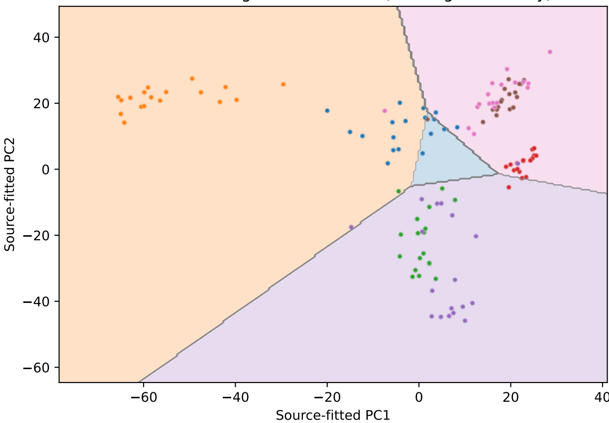
Original classifier on PCA plane; target points Slice/full-head agreement: 52.2% (not target accuracy)
