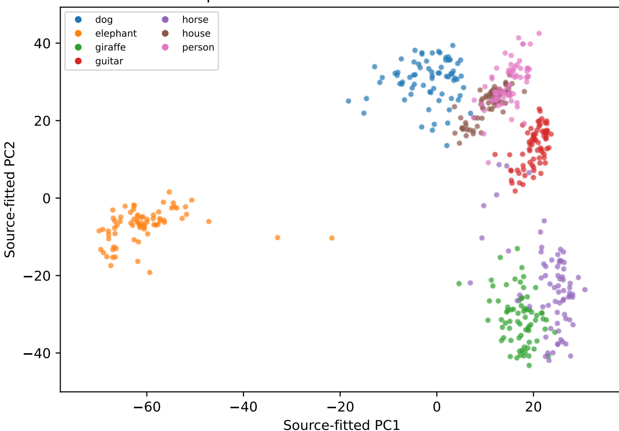
Original classifier on PCA plane; target points Slice/full-head agreement: 38.7% (not target accuracy)
