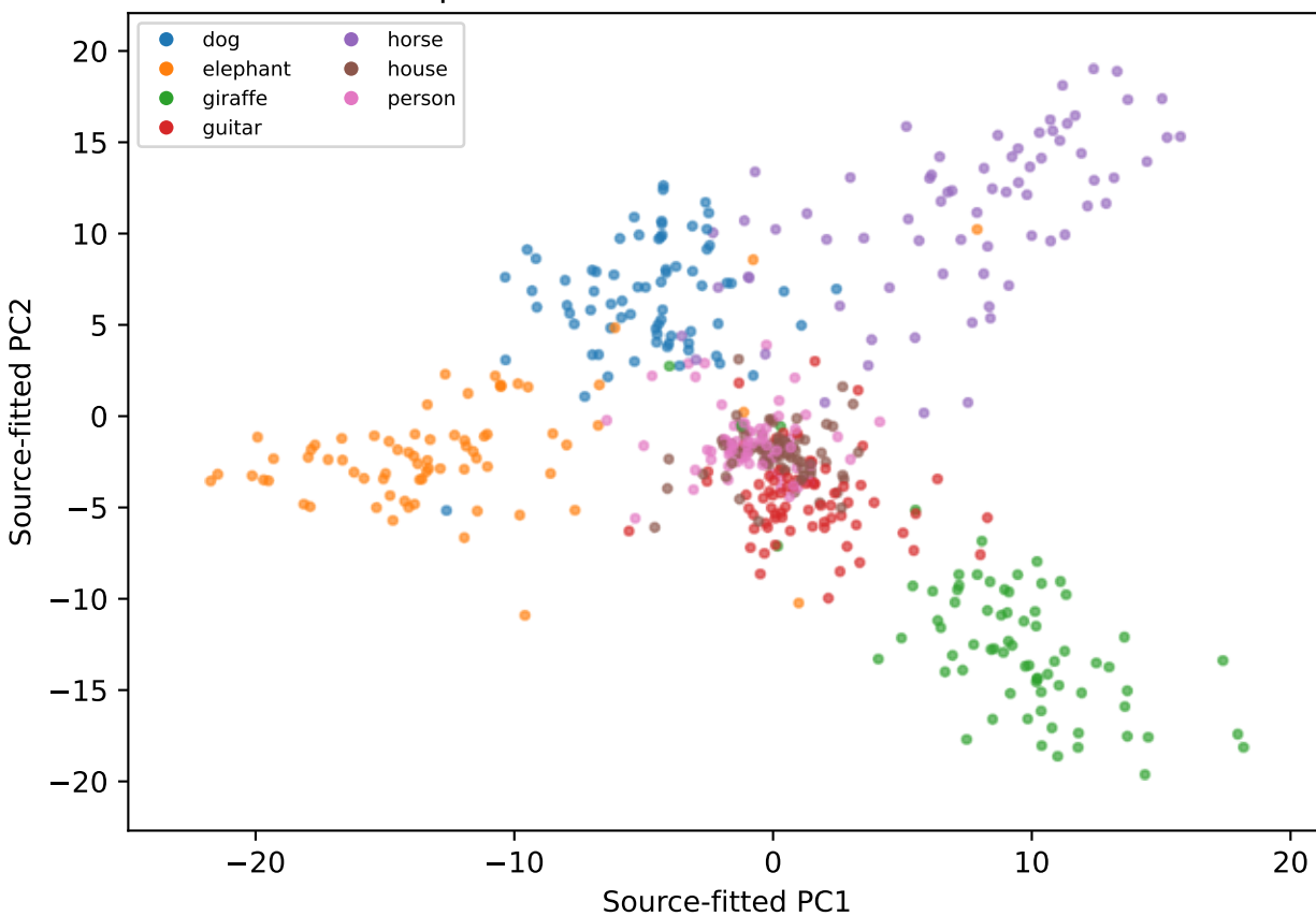
Original classifier on PCA plane; target points Slice/full-head agreement: 41.1% (not target accuracy)
