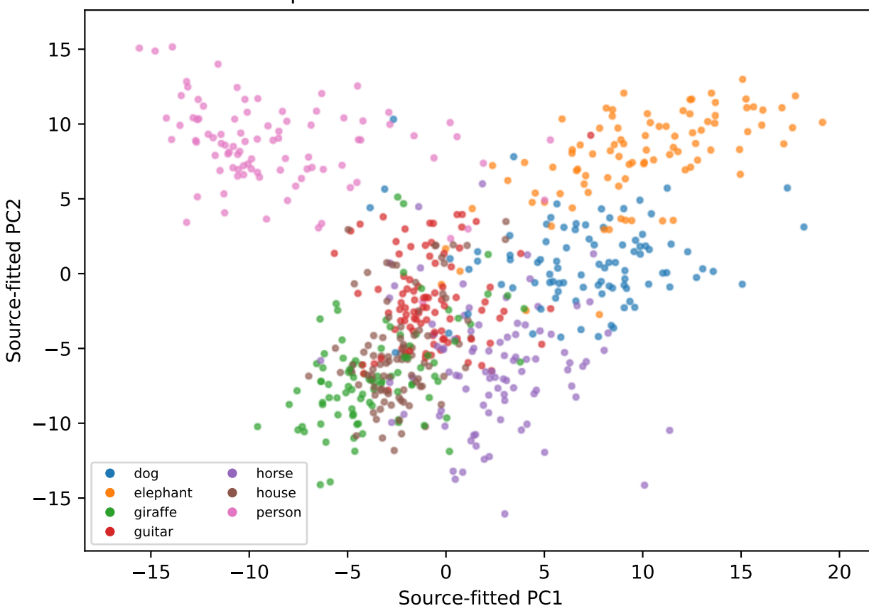
Original classifier on PCA plane; target points Slice/full-head agreement: 49.7% (not target accuracy)
