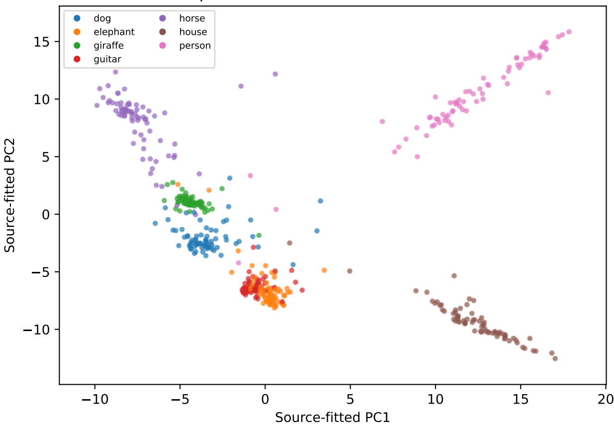
Original classifier on PCA plane; target points Slice/full-head agreement: 65.1% (not target accuracy)
