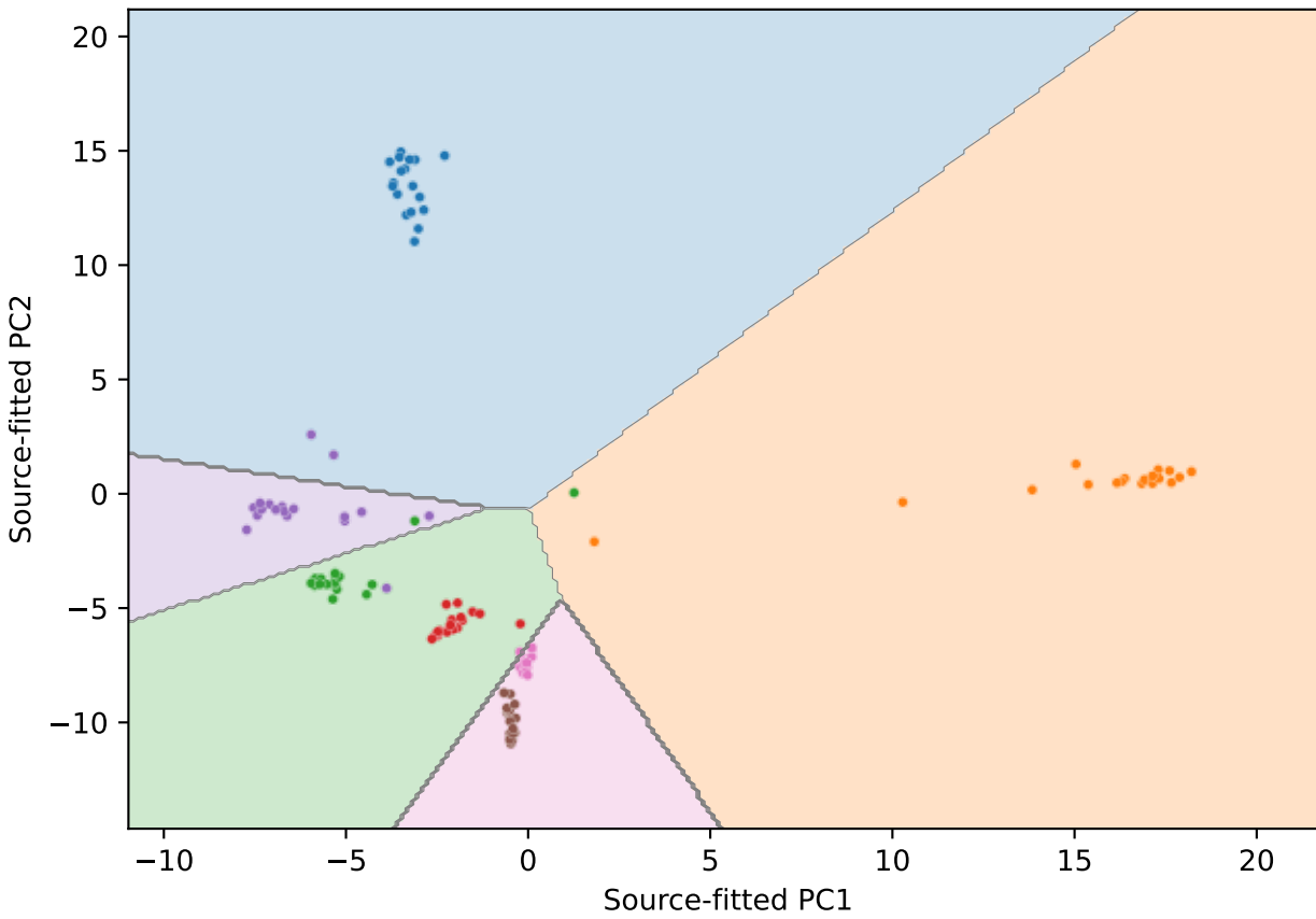
Original classifier on PCA plane; target points Slice/full-head agreement: 65.7% (not target accuracy)
