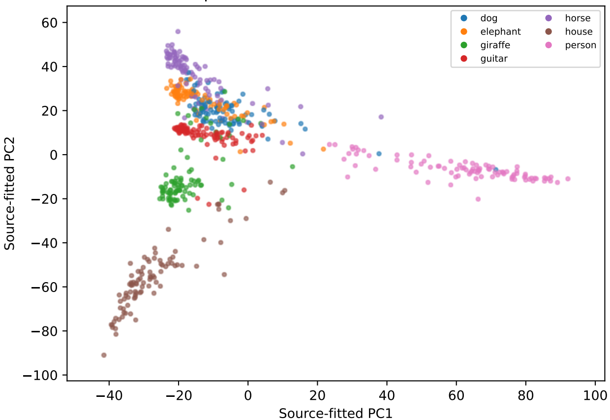
Original classifier on PCA plane; target points Slice/full-head agreement: 21.6% (not target accuracy)
