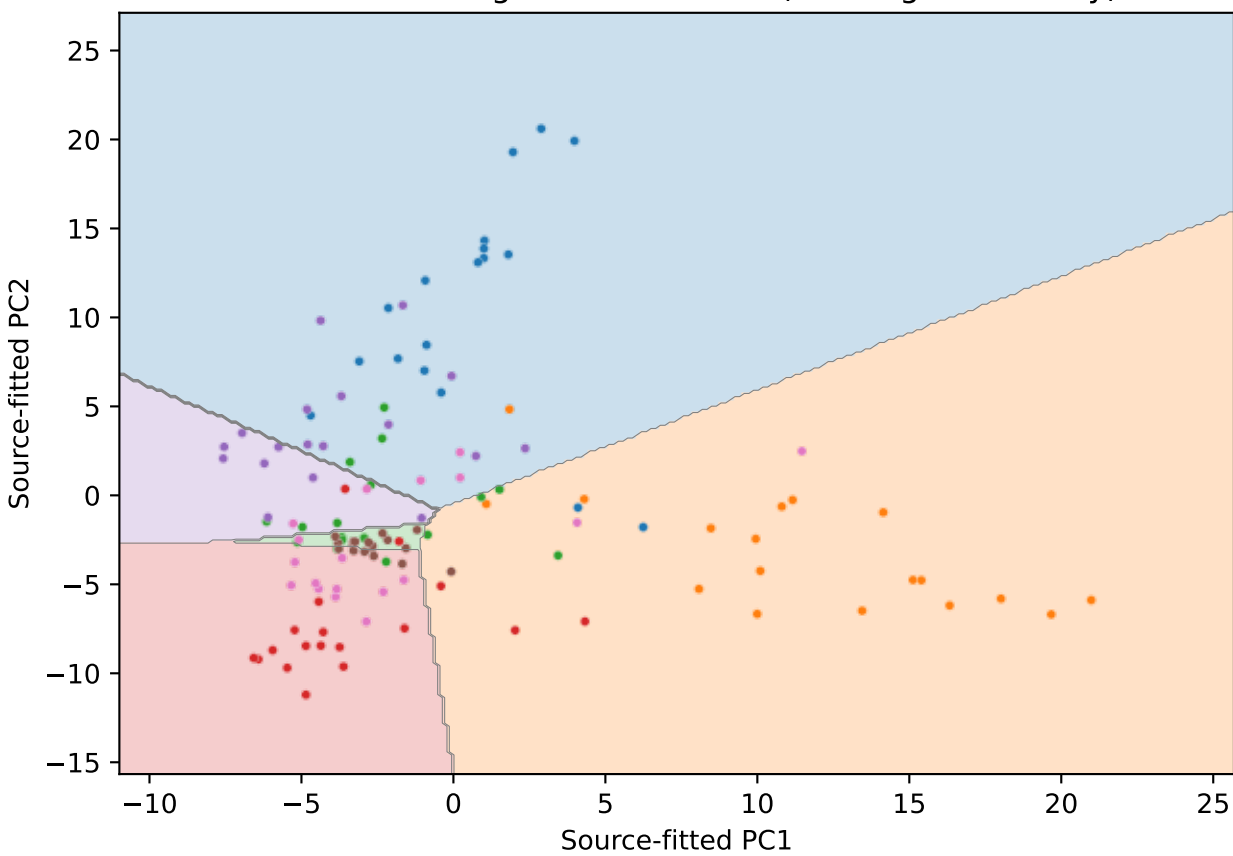
Original classifier on PCA plane; target points Slice/full-head agreement: 47.6% (not target accuracy)
