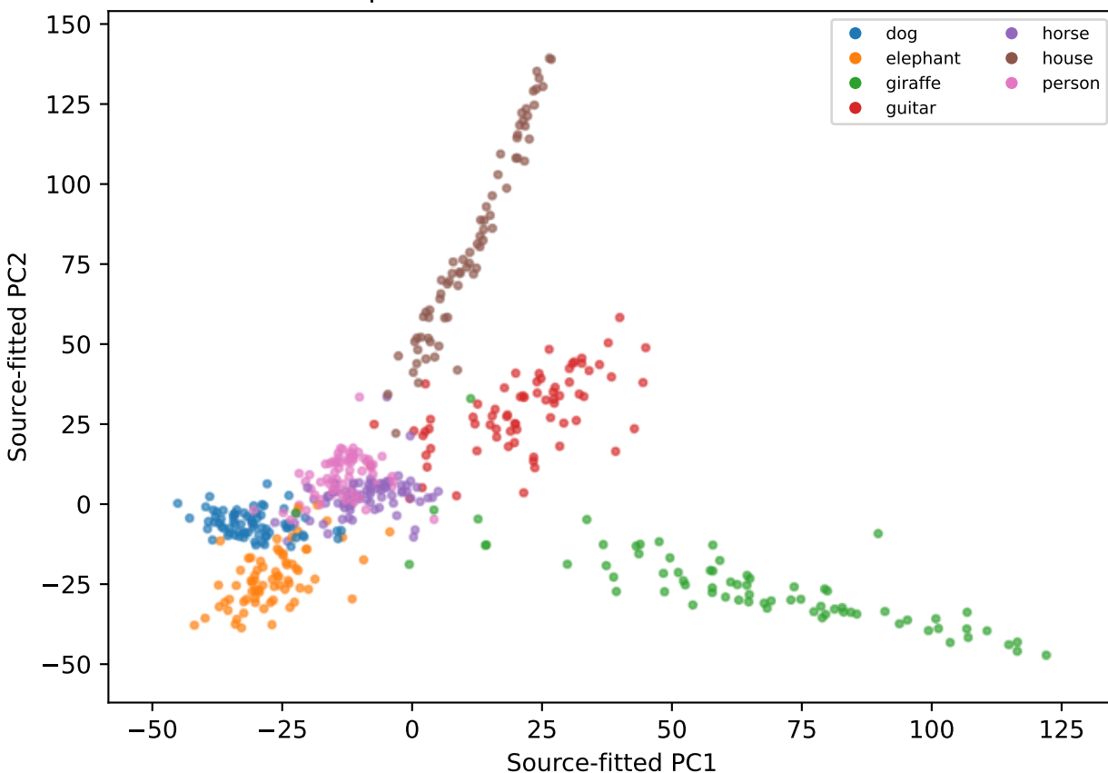
Original classifier on PCA plane; target points Slice/full-head agreement: 40.4% (not target accuracy)
