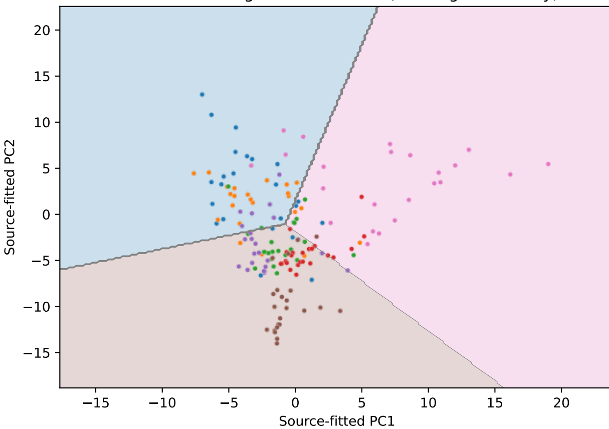
Original classifier on PCA plane; target points Slice/full-head agreement: 20.5% (not target accuracy)
